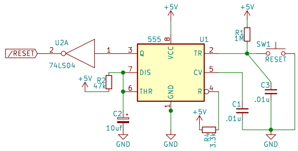
Auto-Reset Circuit
