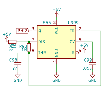
Slow Oscillator
