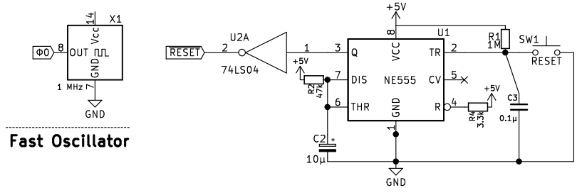
Auto-Reset Circuit
