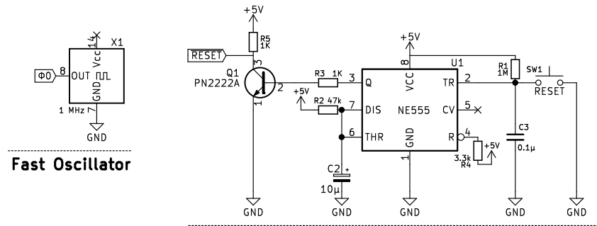
Auto-Reset Circuit
